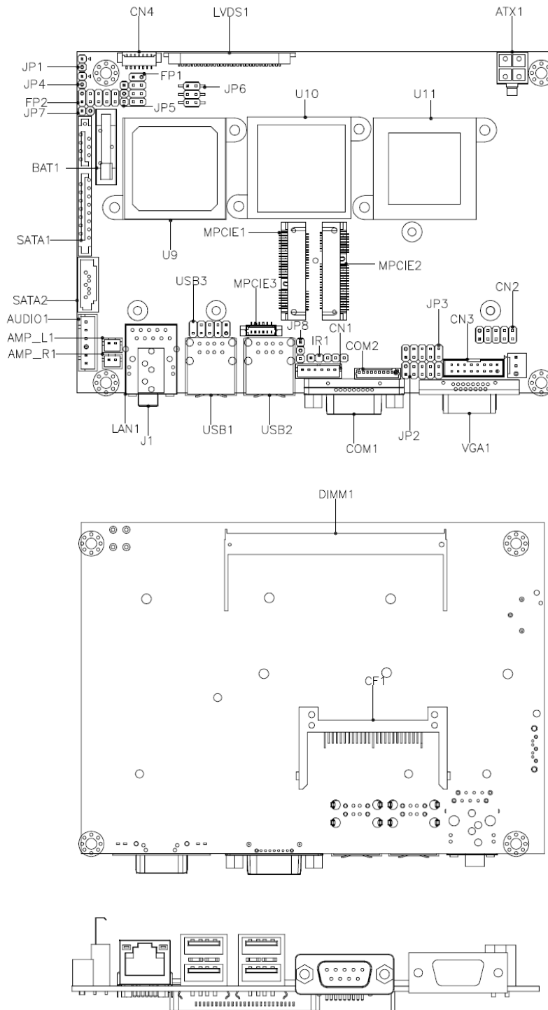
Figure 4 Jumper and Connector Locations
