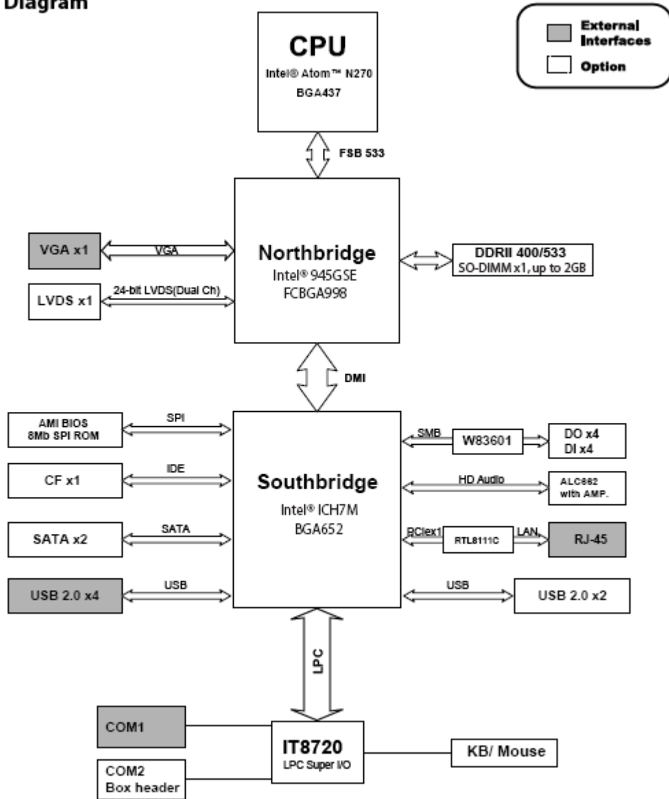
Figure 1 Block Diagram
