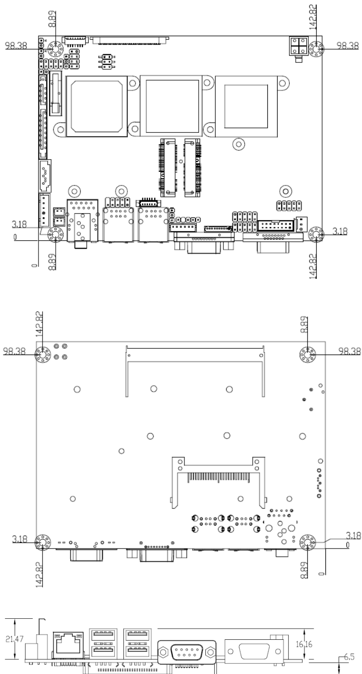
Figure 2 Mechanical Dimensions
